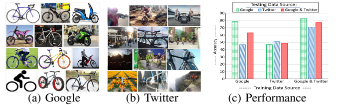
Fig. 1. The significance and challenges in collecting a diverse and informative set of images for dataset construction. (a),(b) Few top-ranked images from Google and Twitter for query 'Bike'. (c) Accuracy of a classifier (10 classes and 400 per class) for different combinations of train and test data.
