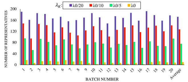
Fig. 6. Number of diverse representatives selected in 20 batches (batch size: 200) of aeroplane class for different value of regularization parameter \lambda_k ( \lambda_k = \lambda_0/\mu_k , where \mu_k > 1 and \lambda_0 is computed from the input data [14]). We observe that the number of selected representatives increases with decreasing value of \lambda_k , or increasing value of \mu_k .
