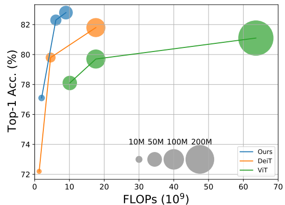
Figure 1: Improvement of our proposed approach over DeiT [35] and ViT [11]. The circle size is proportional to the model size. All models are trained on ImageNet1K from scratch. The results of ViT are referenced from [45].
